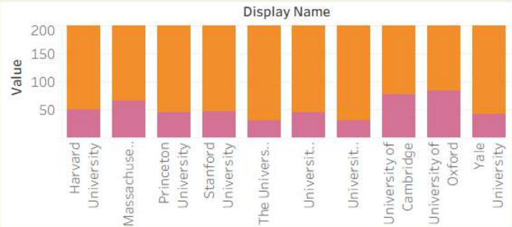
SA-Enrollment Comparisons
