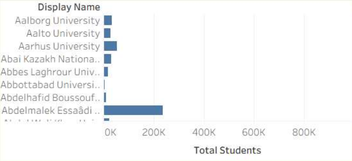
SA-Enrollment Comparisons
